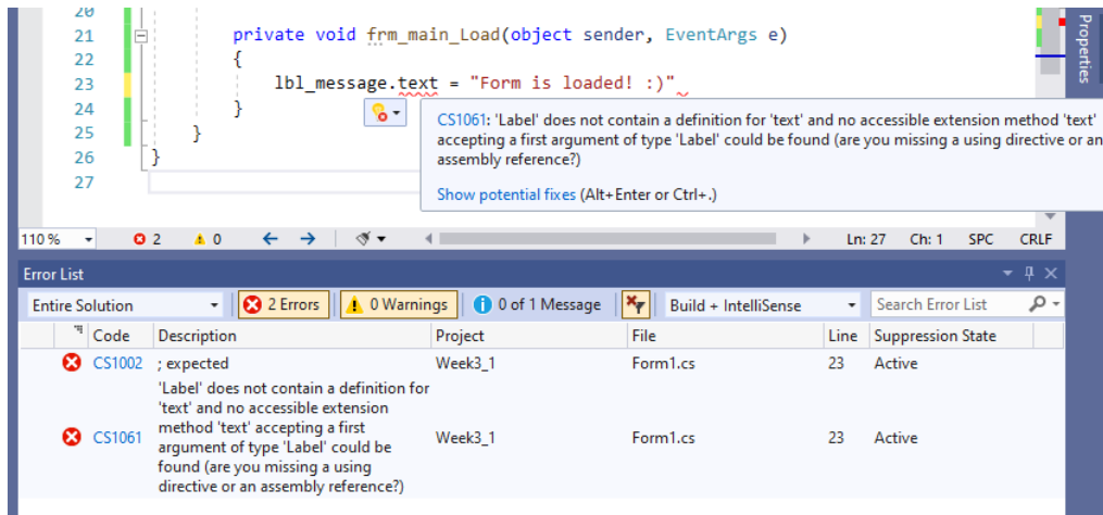
Figure 18. Error messages in the application.
