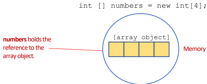
Figure 9. Location assigned in the memory for the array object.
