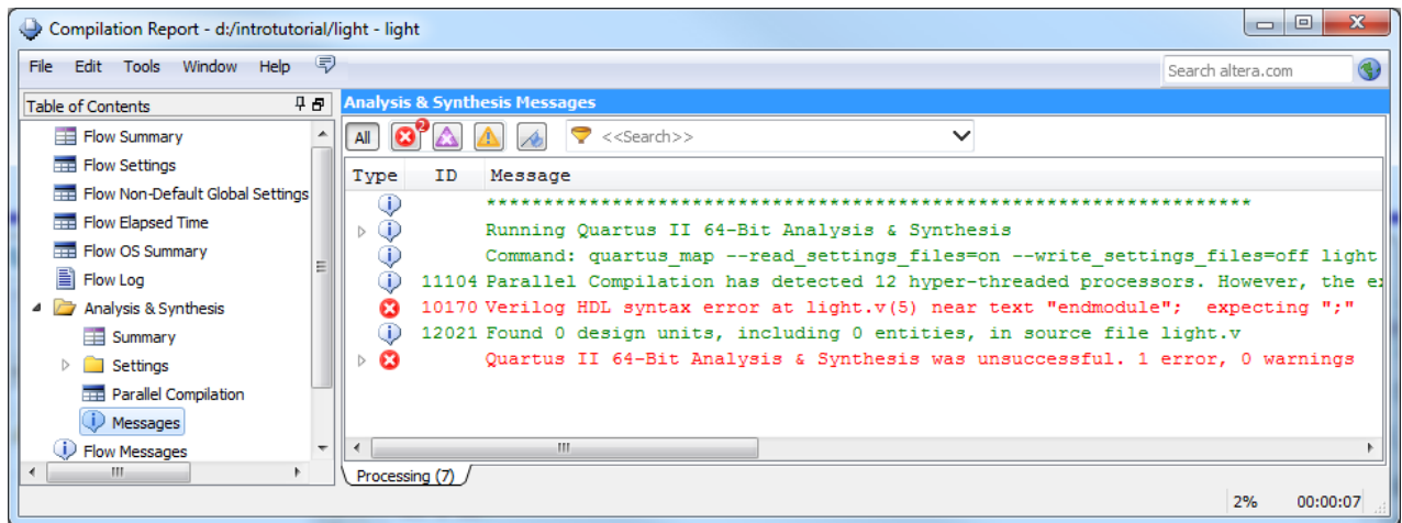
Figure 21. Error messages.
